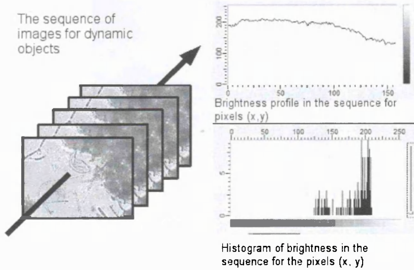
Figure 7. Determination of the background pixel values
