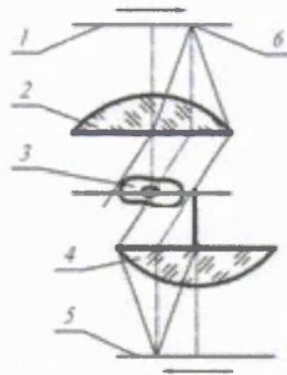
Figure 2. Scheme sensing an object in a microscope with a displaced optical axis
