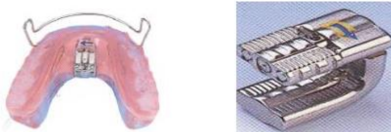
Figure 84. Weise screw in Wunderer activator
