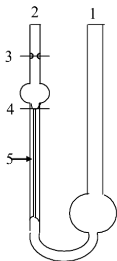
Figure 1. Ostwald viscometer
