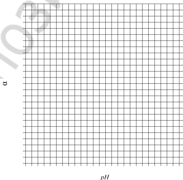
Figure 1. Dependence of the degree of swelling of the protein on the pH of the medium
