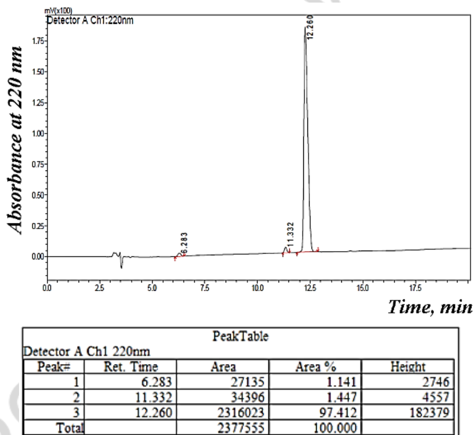
Figure 4.6. An output of HPLC chromatograph with the information on peaks: retention time, absolute area, percent of the area, the height
