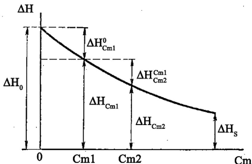
Figure 1.1. Heat effects of the dissolving
