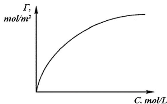
Figure 4.4. The isotherm of adsorption according to the Freundlich theory
